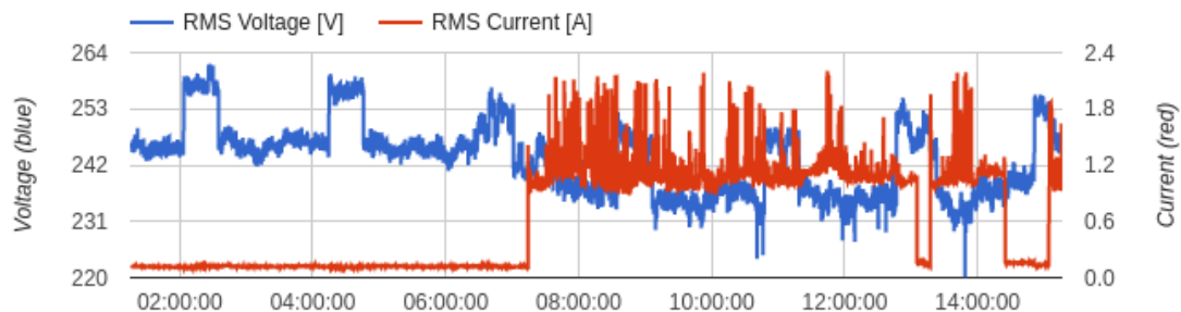
Figure 7–4 The preview of the visualised data from the data stream displaying 14 hours of data; it can be seen when the appliance was in standby mode (red) or the periodical fluctuations of the mains voltage (blue)
