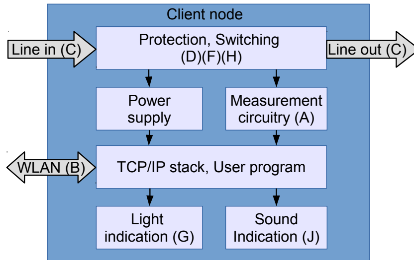
Figure 6–2 The block diagram of a client node of a proposed system, including hardware requirements
