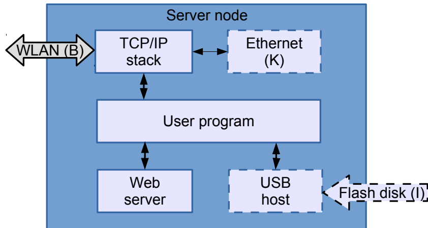
Figure 6–1 The block diagram of a server node of a proposed system, including hardware requirements
